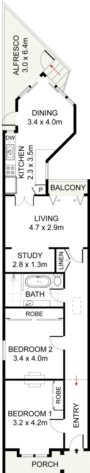
GROUND FLOOR
